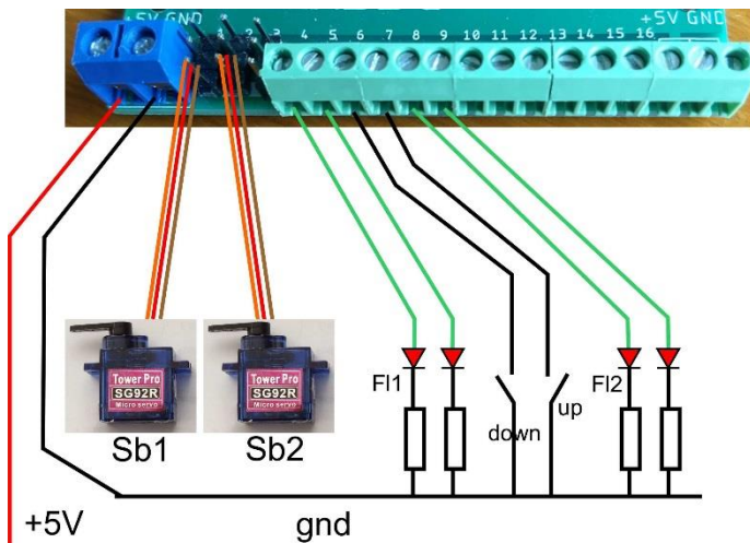
Railway crossing controlled manual with 2 switches. No DCC required
